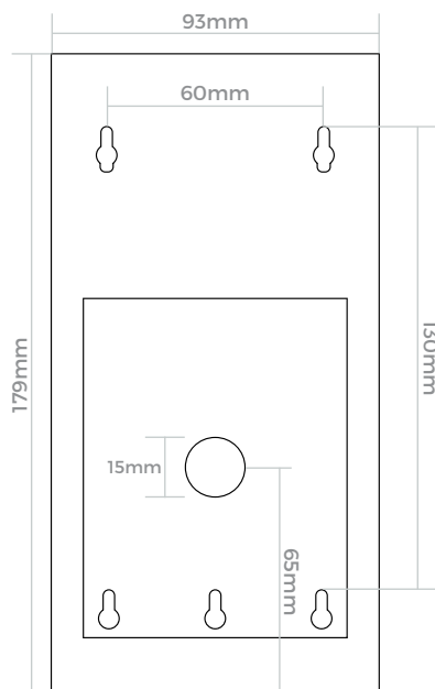
Wall mounting dimensions
