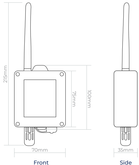
MPD dimensions
